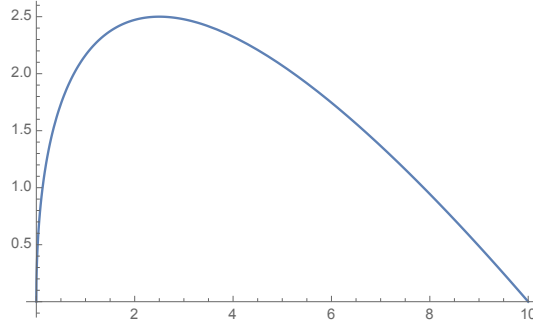
Figure 1: Best reply function
