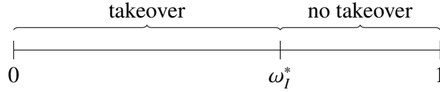
Figure 2: The \omega_I -Type Space with Cutoff Type \omega_I^*
