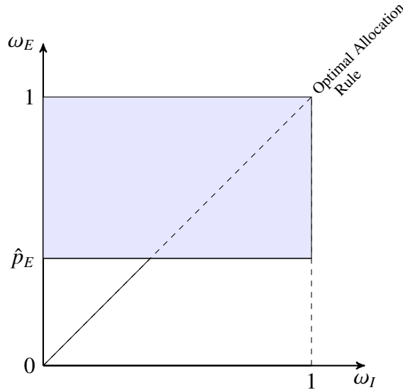
Figure 3: Optimal Allocation vs. Pooling Equilibria
