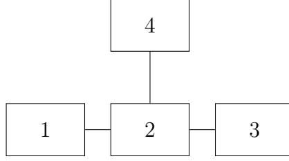
Figure 2: Tree Example
